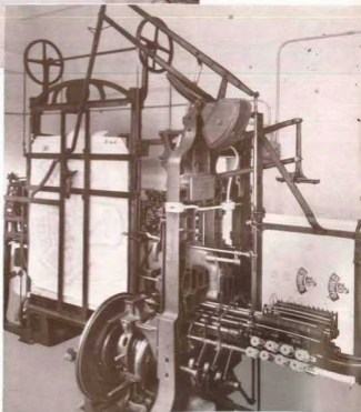
SWISS EMBROIDERY PATTERN MACHINE
